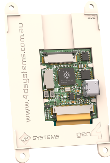
gen4-RP2350-32CT Rear
